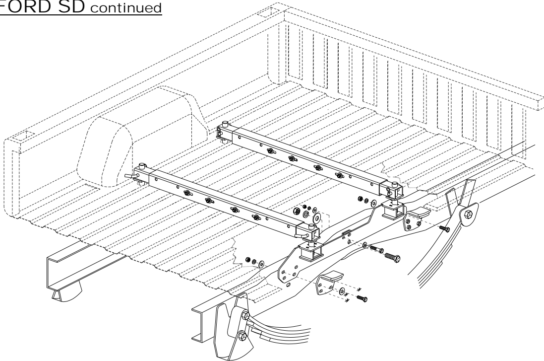
Cutaway view, of Mounting Plate installation
