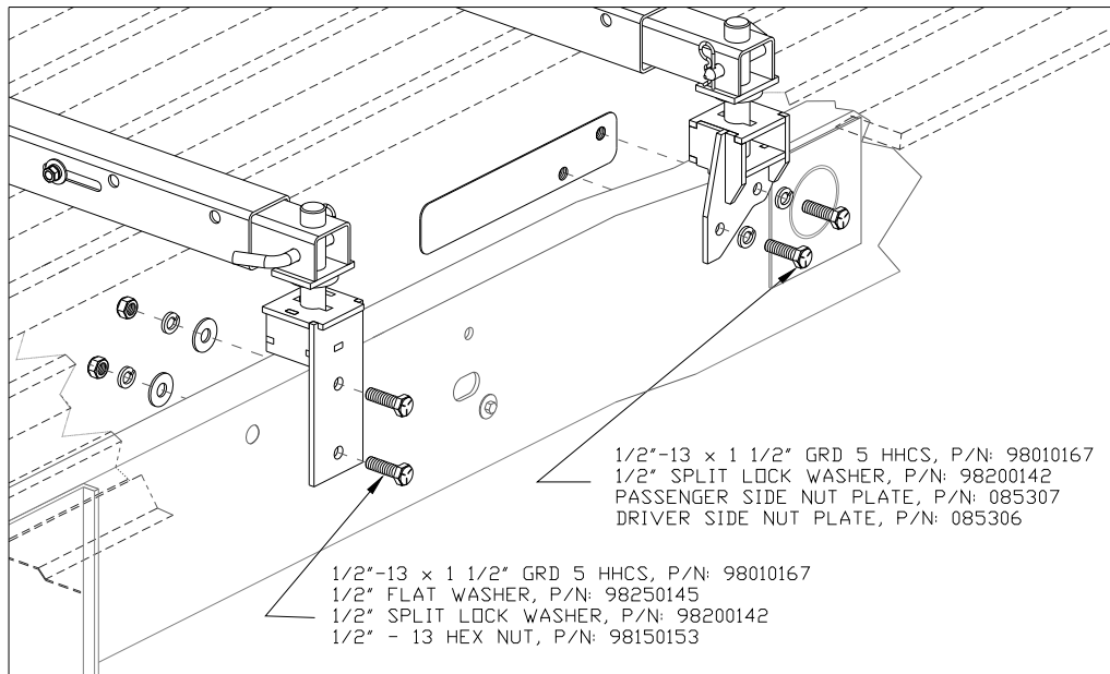
Base Rail Detail View Illustration
