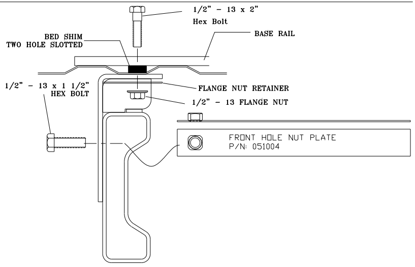
FRONT BASE RAIL AND BRACKET
