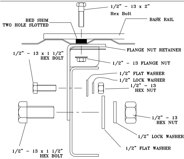
REAR BASE RAIL AND BRACKET
